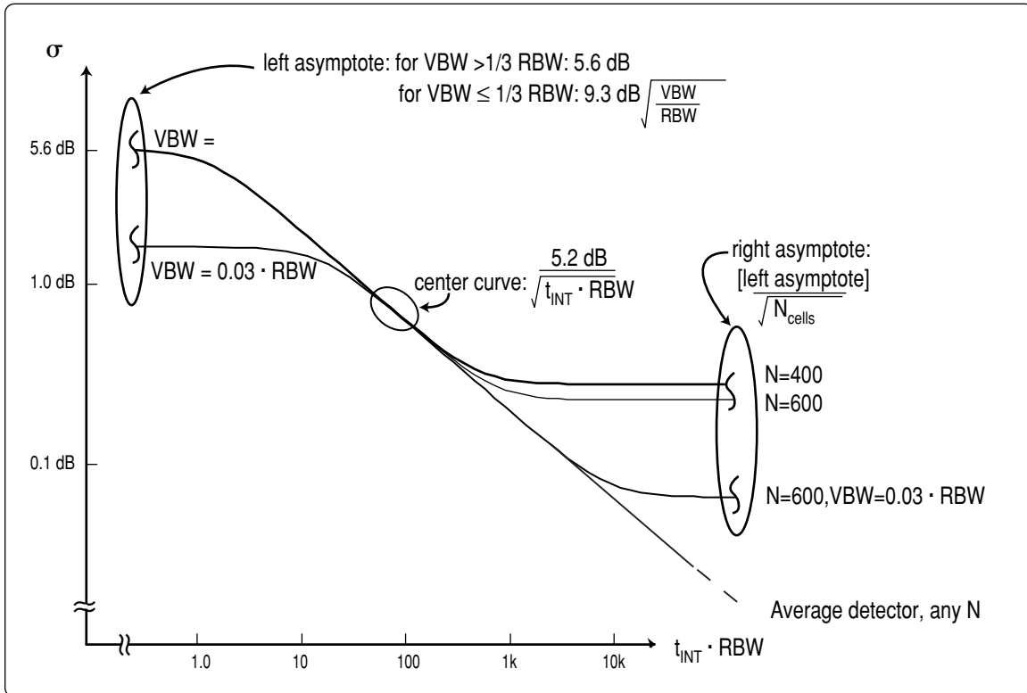
Figure 10. Noise measurement standard deviation for log-response spectrum analysis depends on the sweep-time/RBW product, the VBW/RBW ratio, and the number of display cells.
